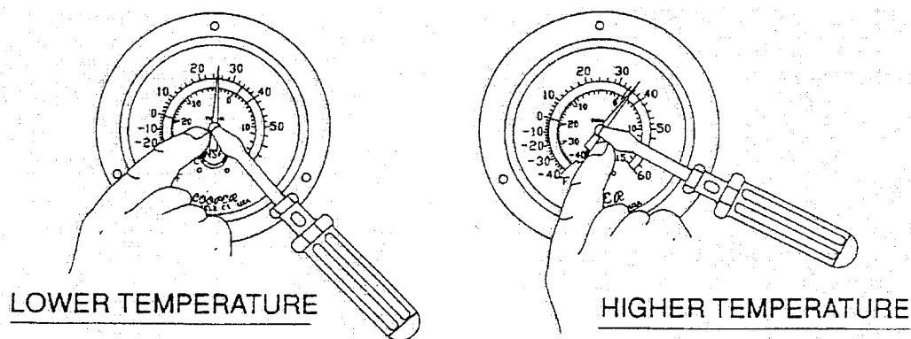
Figure 4.1 – Thermometer Calibration
